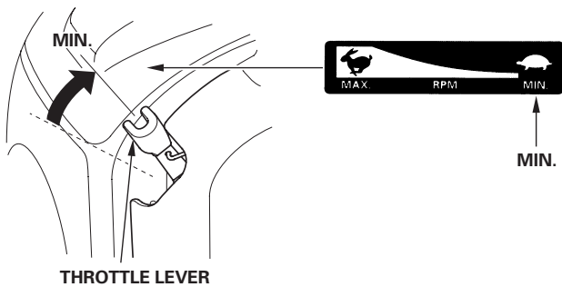
THROTTLE LEVER
